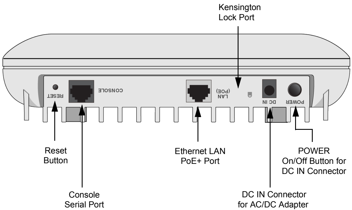
Figure 3. Rear Panel
