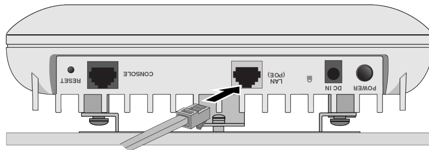
Figure 23. Connecting an Ethernet Cable to the LAN Port
