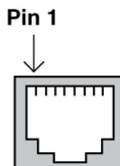
Figure 33. Pin Layout for RJ45 Connector on the Ethernet Port
